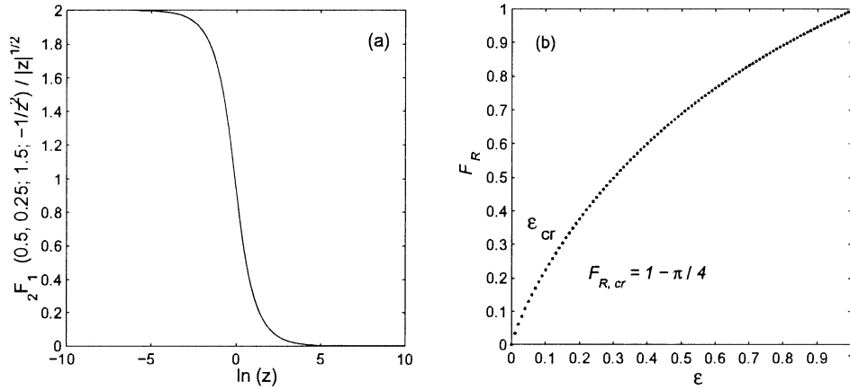
Figure 4. (a) The term containing the hypergeometric function appearing in both evolution equations, (20) and (29), with z = |\xi|/(\epsilon h) . Its limit for z \rightarrow 0 is finite, proving that this term does not represent a singularity. (b) The filling fraction F_R as a function of the expansion parameter \epsilon for the initial condition h(\xi) = 1 + \xi^2 used throughout this paper. The critical filling fraction and the corresponding critical value of \epsilon are marked by the dashed lines.
